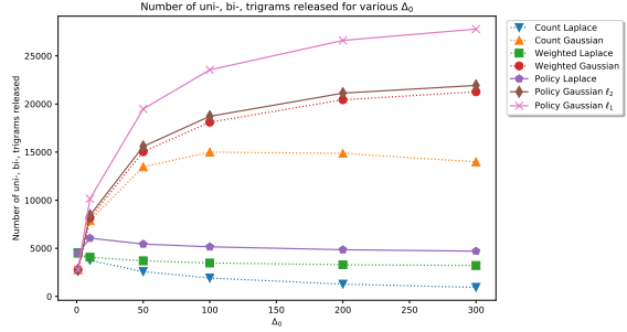
Figure 11: Count of unigram, bigrams, and trigrams released at various values of \Delta_0 for parameters \varepsilon = 3 , \delta = \exp(-10) .
